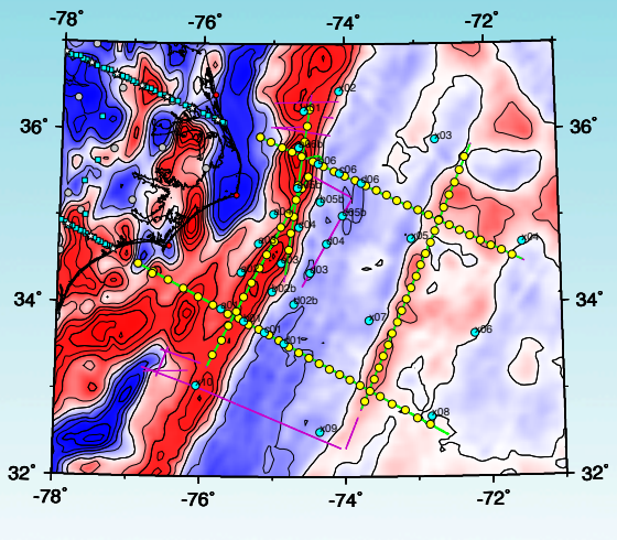
Magnetic Anomaly (nT)
