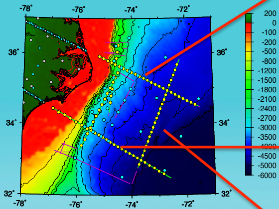
Bathymetry (m)
