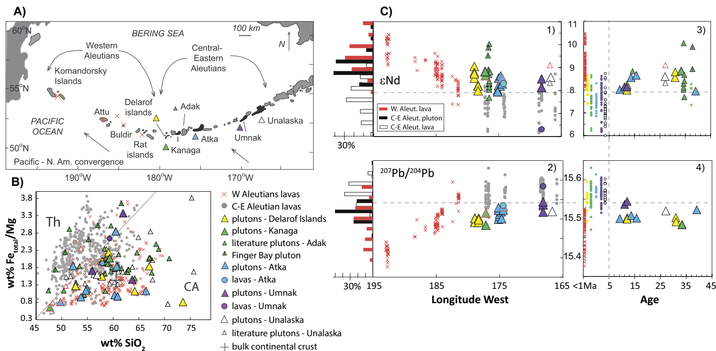
A) Schematic map of the Aleutian island arc, sampled areas are highlighted in black. B) \text{wt\% SiO}_2 versus \text{Fe}/\text{Mg} ratio of studied Aleutian igneous rocks. By convention, the \text{Fe}/\text{Mg} ratio is calculated using \text{wt\% MgO} and \text{FeO} , with all \text{Fe} as \text{FeO} . C) Present-day Nd and Pb isotope ratios of Aleutian igneous rocks vs. longitude and vs. age. Circles are central and eastern Aleutian volcanics: Yellow = Rat and Delarof Islands, Green = Adak and Kanaga, Blue = Atka, Purple = Umnak, White = Unalaska. Error bars are smaller than the symbols. In 3) and 4), the Holocene volcanics are separated by location only without age differences. Figures from Cai et al., Earth Planet Sci. Lett. 2015.
