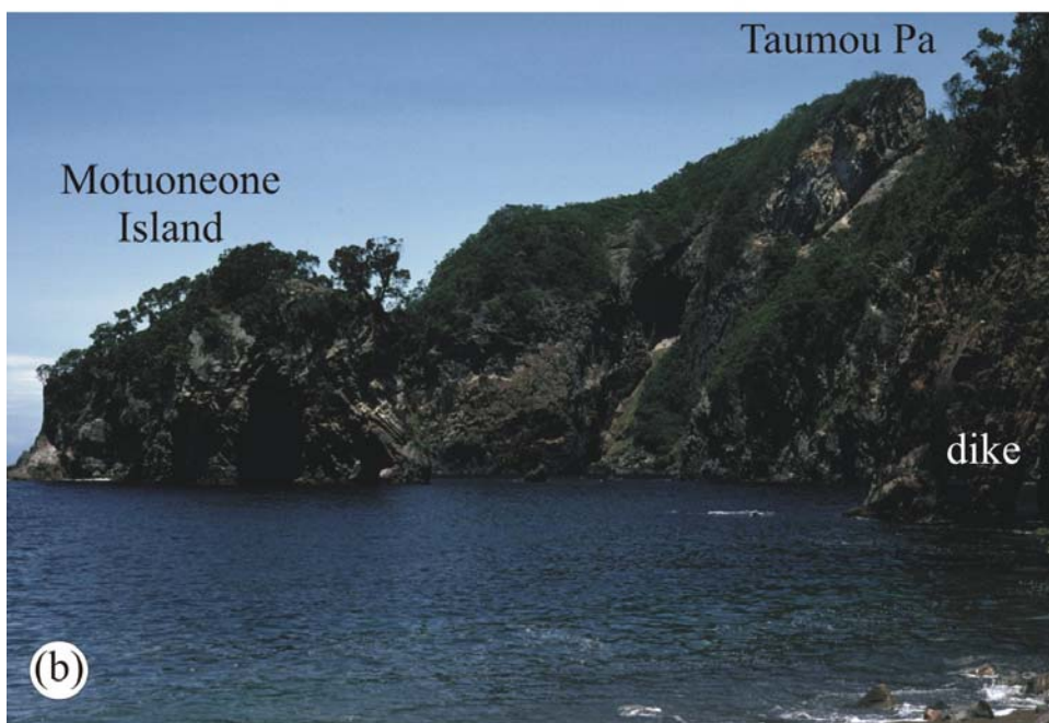
Figure 6. Viewpoint 3: Oturu Bay. (a) Oturu pumice cone, cut by a dike feeding a 55 ka lava flow. (b) View from the beach below the Oturu pumice cone, looking towards the south. Note the steep outboard dip of the Taumou lava. An older lava has been eroded back to form Motuoneone Island.
