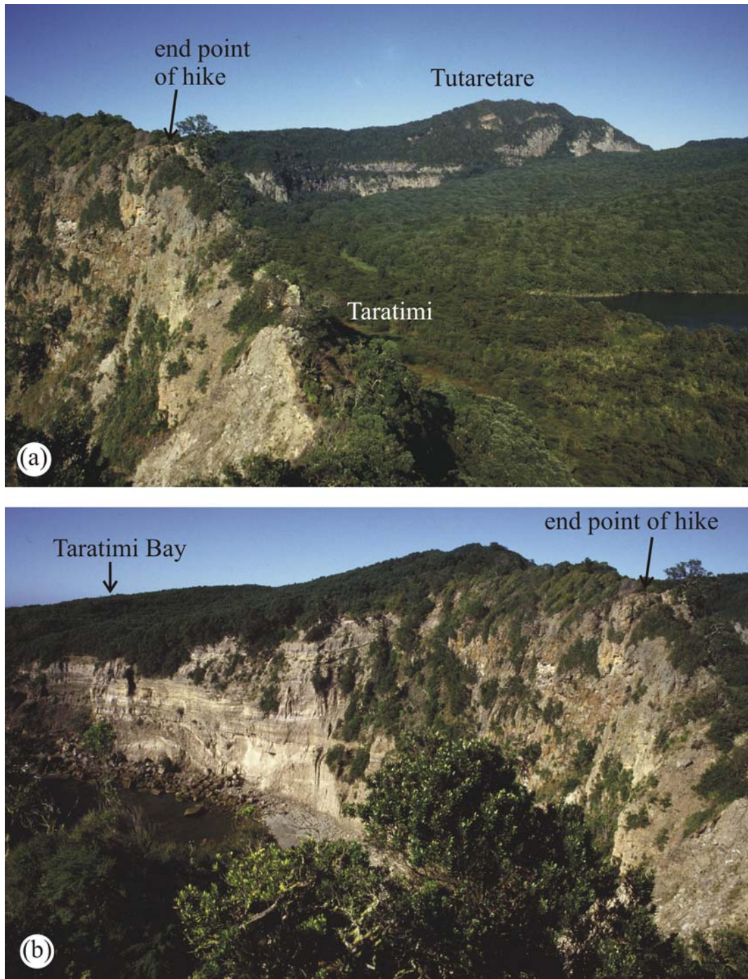
Figure 16. Two views from the slopes of Taumou hill, to show the setting of the end point to the hike. Note the narrowness of the caldera rim in this section. Part (b) shows the pyroclastic section in Taratimi Bay seen from the boat and shown in Fig. 5(a).
