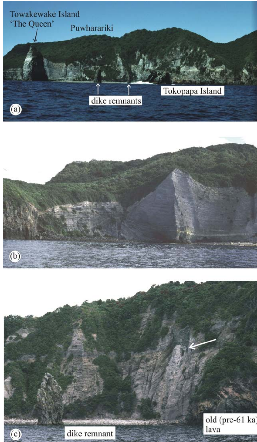
Figure 8. Viewpoint 5: Orongatea Bay. (a) General view, showing dike and lava flow remnants forming offshore islets. (b) Orongatea pumice cone at the eastern end of the bay. (c) Complex pyroclastic deposits at the western end of the bay, resting on an old lava and cut by a dike remnant (arrowed).
