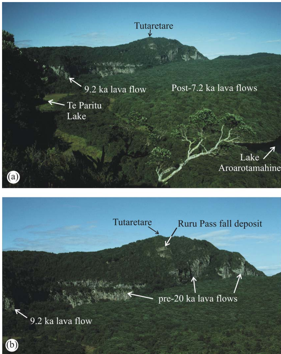
Figure 14. View from the end-point of the hike, looking southwest. (a) Wide view; note the lobes of the young lavas outlined by vegetation growth on the floor of the caldera. (b) Detail of Tutaretare showing the older lavas, draped by a lobe of the 9.2 ka lava flow. Note that the upper one-third to one-half of Tutaretare represents a cone of the Ruru Pass fall deposit erupted during the opening stages of the 7.2 ka eruption. To the left, this fall deposit passes into an intensely welded, mildly rheomorphic tuff (Houghton et al., 1985a).
