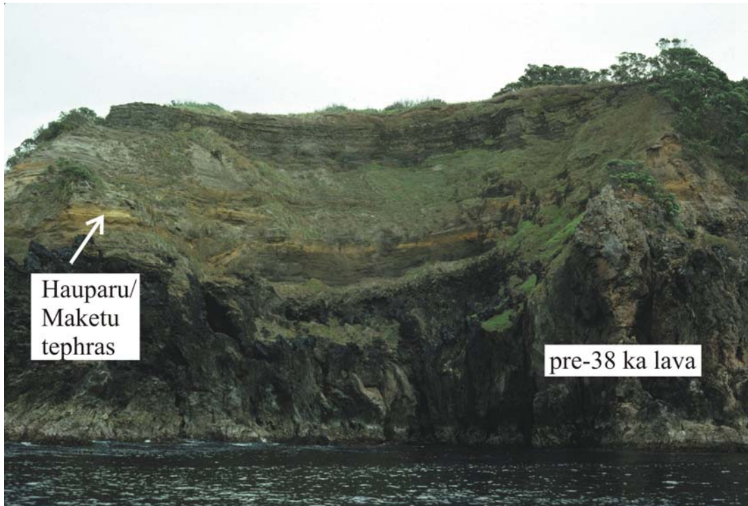
Figure 4. Viewpoint 1: Tauranga Point. The mainland-derived Hauparu and Maketu tephras serve as ~38 ka marker plane to provide a minimum age for many parts of the island.
