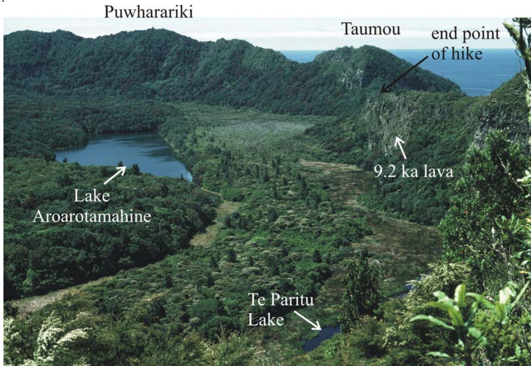
Figure 13. View from the rim track towards the northeast, showing the eastern floor and rim of the 7.2 ka caldera.
