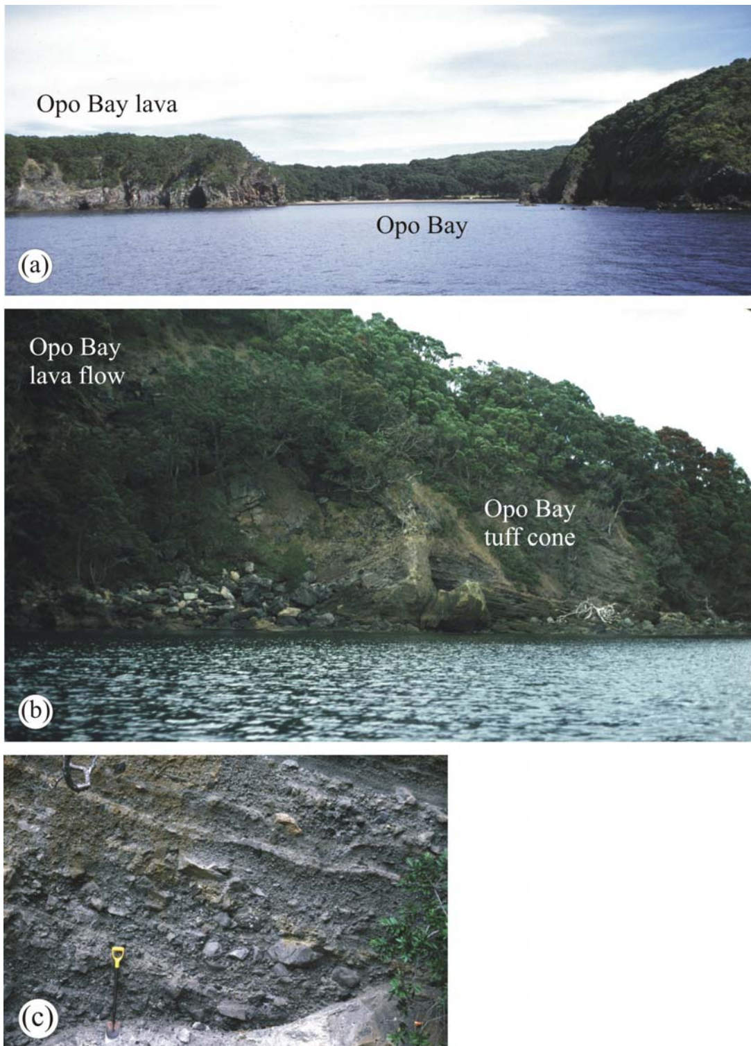
Figure 12. Viewpoint 9: Opo Bay. (a) View into Opo Bay, showing the Opo Bay lava flow to the left. Note that prior to the 7.2 ka eruption, there was a channel between the Opo Bay lava and the rest of the island. (b) View of the Opo Bay lava overlying the northern rim of the earlier syn-eruptive tuff cone. (c) Poorly sorted deposits on the Opo Bay tuff cone on its outer slopes, occurring at the southern end of Opo Bay beach.
