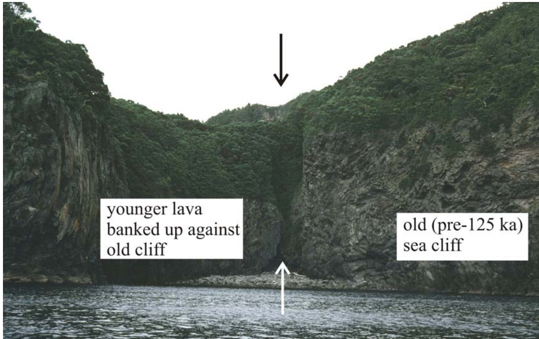
Figure 7. Viewpoint 4: Turanganui Bay. An extra-caldera lava (Paretao) dated at 33 ka abuts an old sea cliff cut into an undated lava. Arrows mark the contact.
